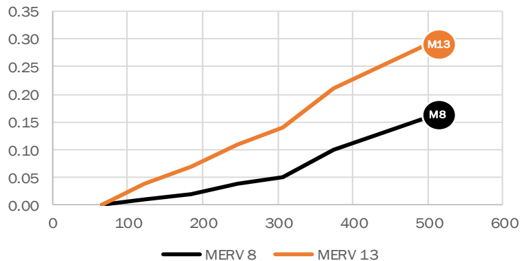
24 x 24 x 2 Resistance vs. Filter Face Velocity
