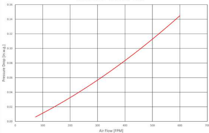
Air Flow MERV 11 - 24 X 24 X 18 - V-bank
